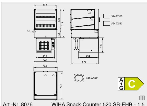
Art.-Nr. 8076 WIHA Snack-Counter 520 SB-EHB - 1.5
