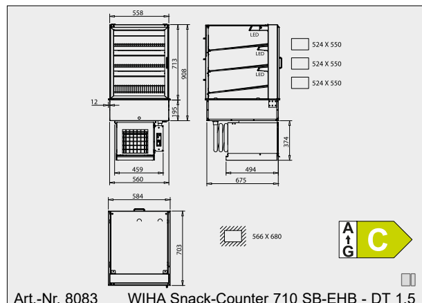
Art.-Nr. 8083 WIHA Snack-Counter 710 SB-EHB - DT 1.5
