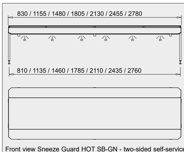
Front view Sneeze Guard HOT SB-GN - two-sided self-service
