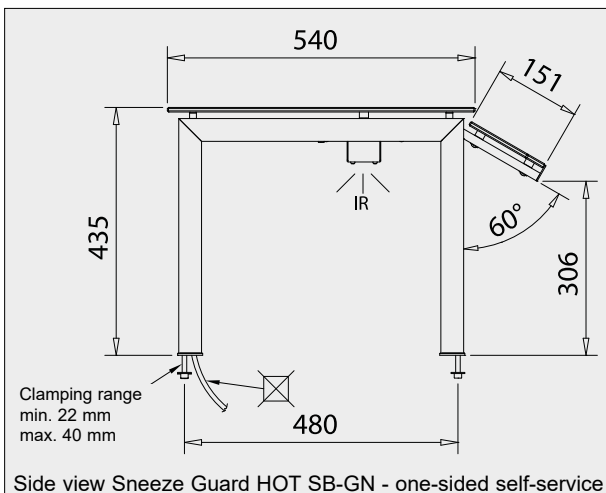
Side view Sneeze Guard HOT SB-GN - one-sided self-service
