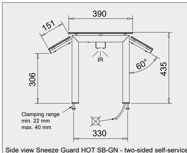
Side view Sneeze Guard HOT SB-GN - two-sided self-service
