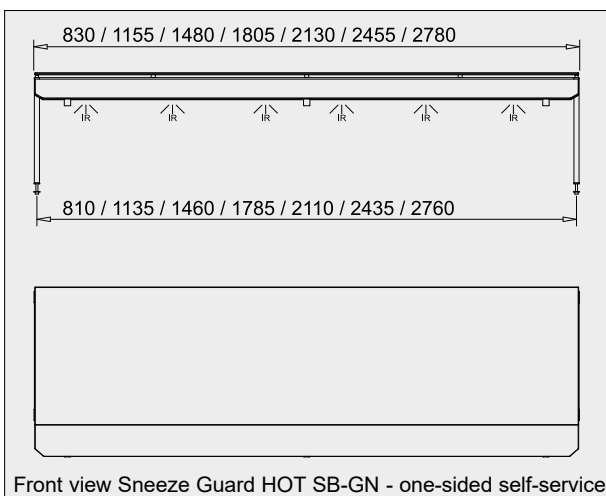
Front view Sneeze Guard HOT SB-GN - one-sided self-service
